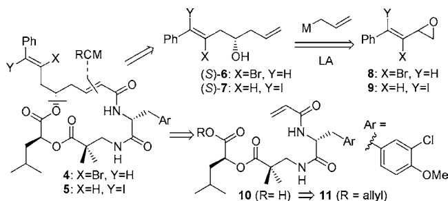
Figure 2. Retrosynthetic analysis of the cryptophycin scaffolds.
