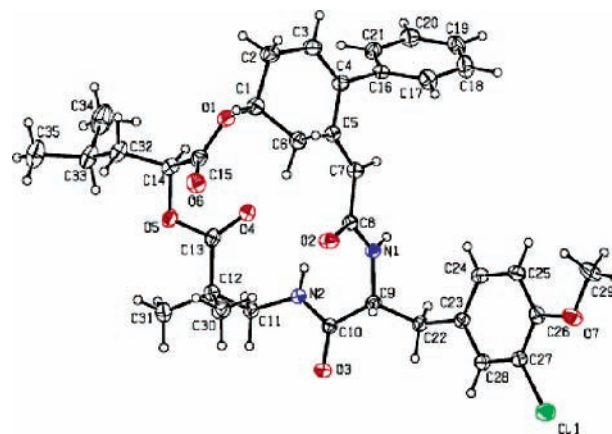
Figure 3. Crystal structure of 22 .
