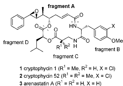
Figure 1. Various cryptophycin structures.
